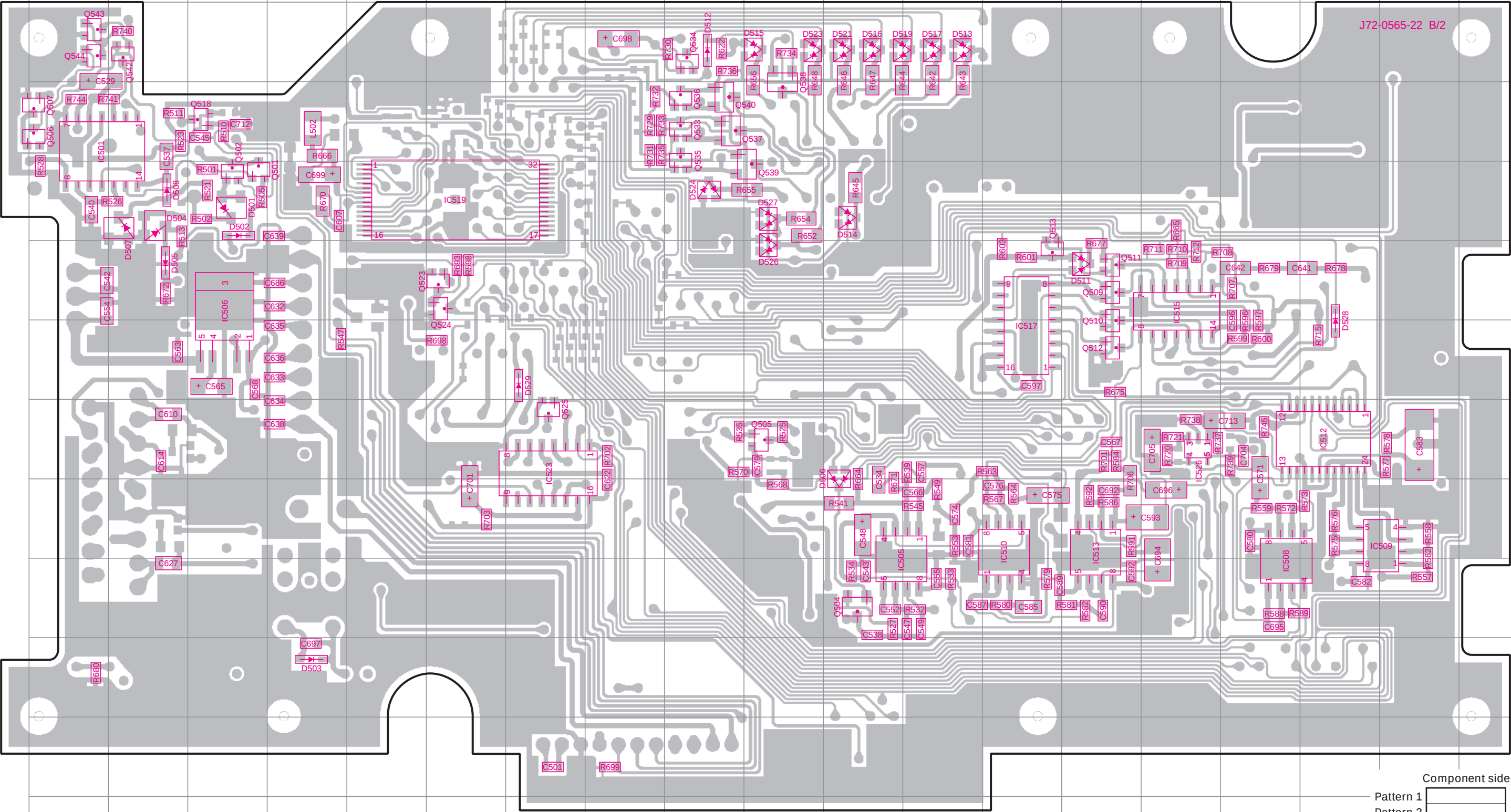
CONTROL UNIT (X57-5600-XX) (B/2) -10 : K -11 : K2 -12 : K3 Foil side view
